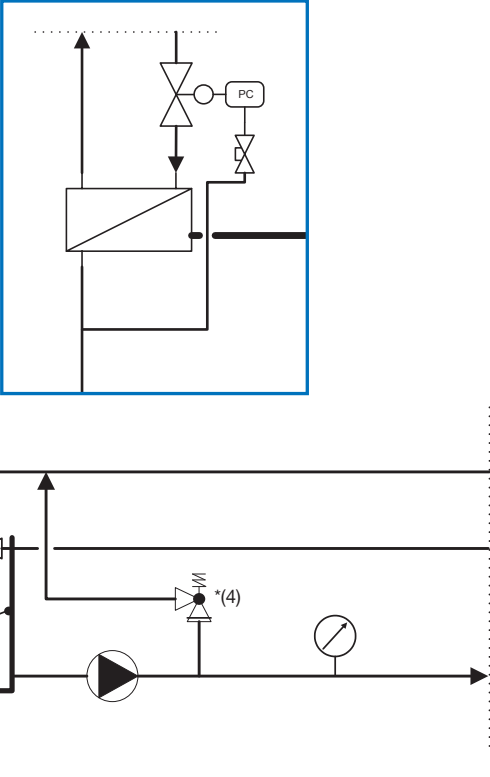
Flow chart with water cooled condenser
