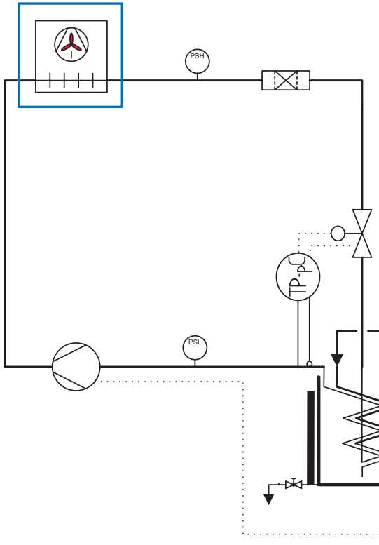
Flow chart with air cooled condenser
